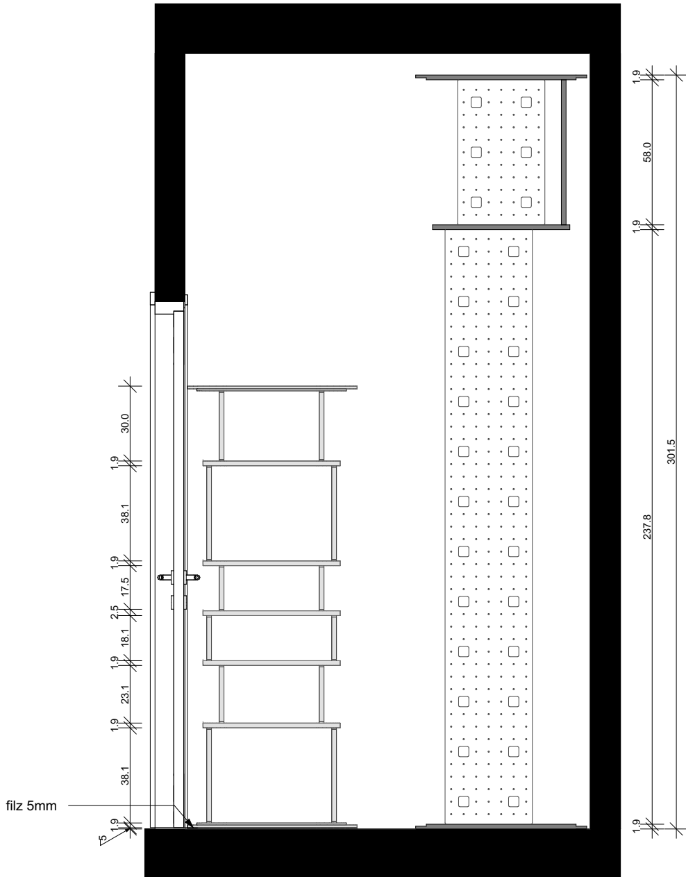
section c-c
