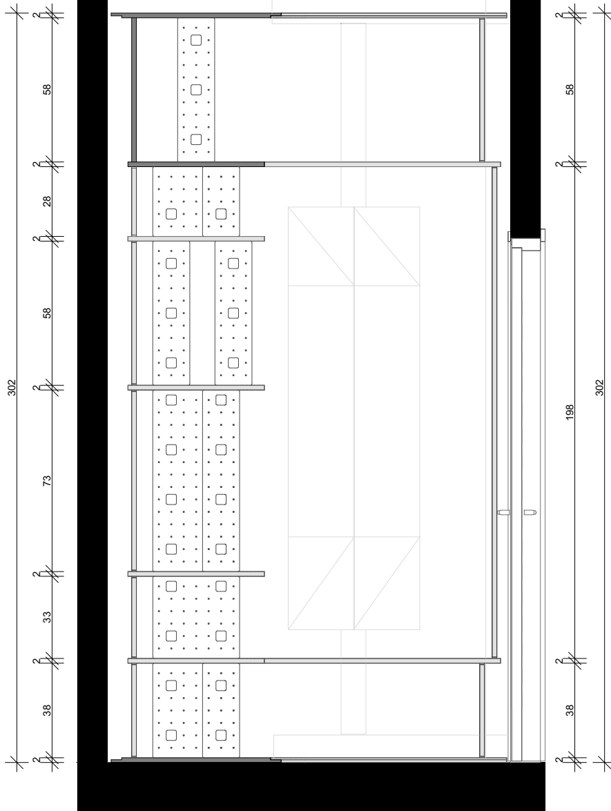
section b-b
